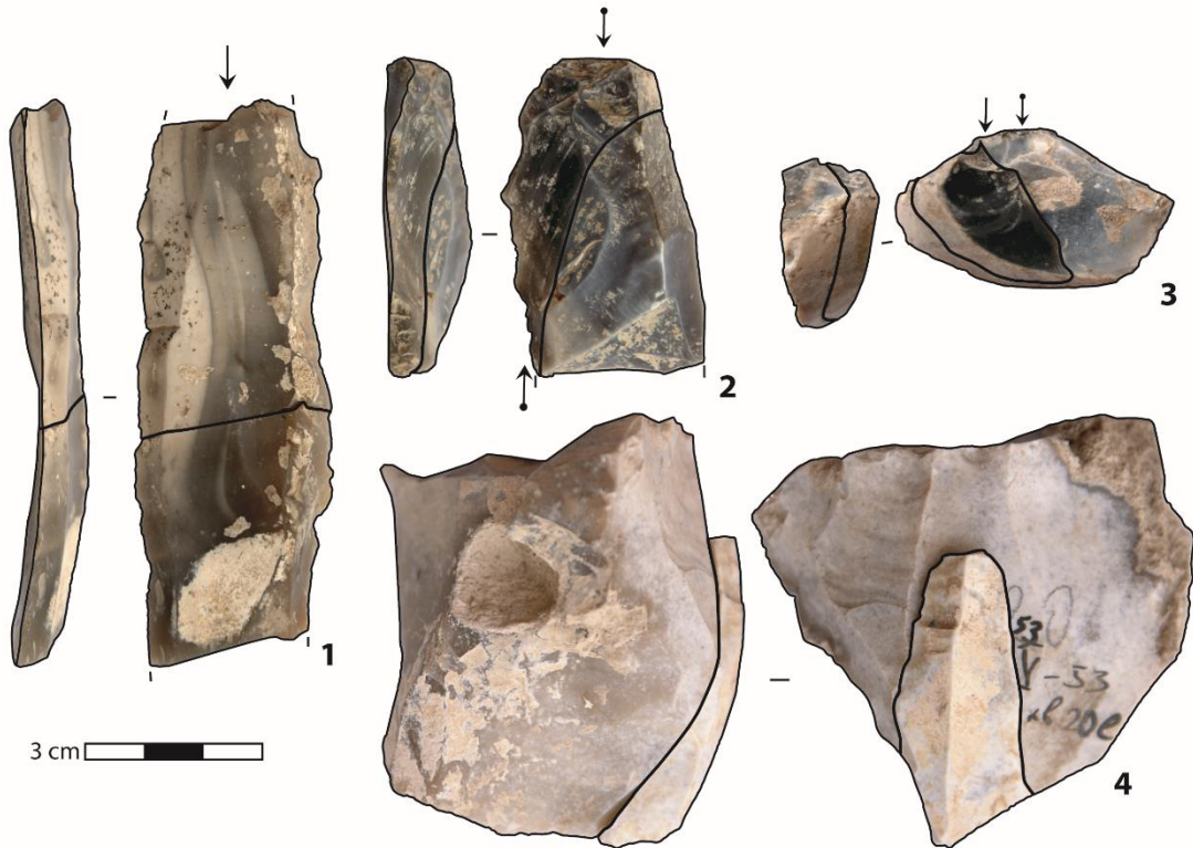
Fig. 11. Molodovo V. Examples of inter-levels refits. 1–2 – Levels 9 and 8 refits; 3–4 – Levels 10 and 9 refits
